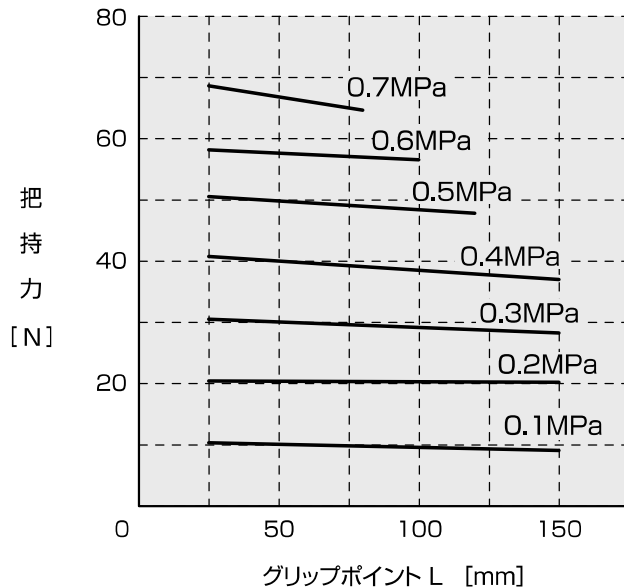
NEOK(F)-20C
