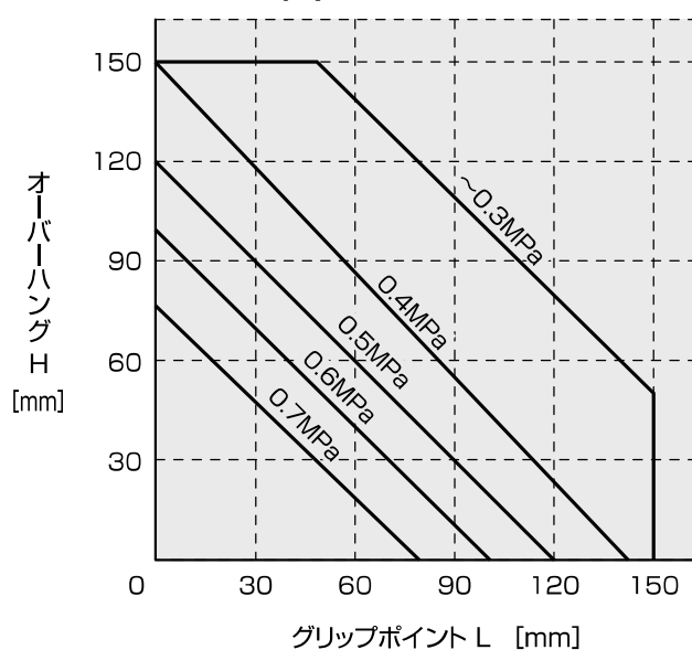
NEOK(F)-20C
