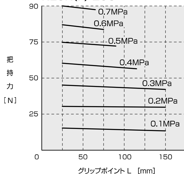
NEOK(F)-20C
