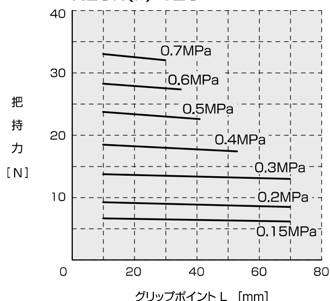
NEOK(F)-12C
