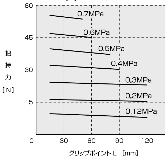
NEOK(F)-16C
