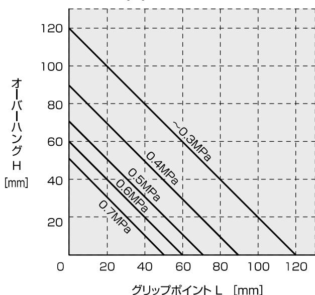
NEOK(F)-16C
