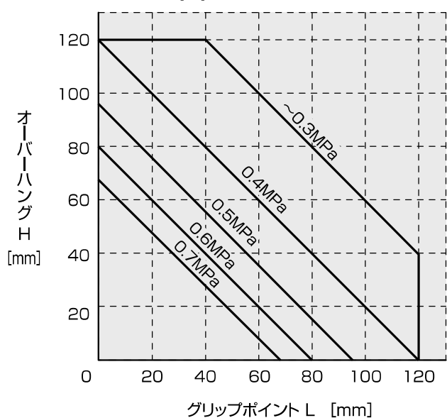
NEOK(F)-16C
